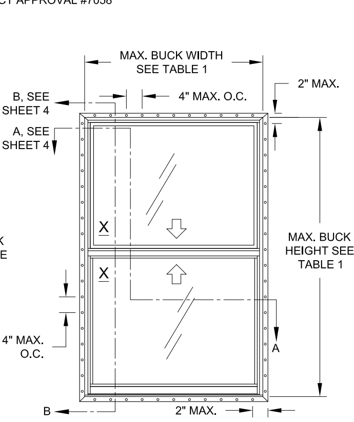
ELEVATION FOR TYP. FIN OR J-CHANNEL FRAME, EQUAL-LITE CONFIGURATION (SIMILAR ANCHOR DIMENSIONS FOR OTHER CONFIGURATIONS)
